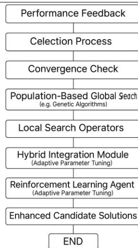
FIGURE 6. Hybrid Metaheuristic Framework
