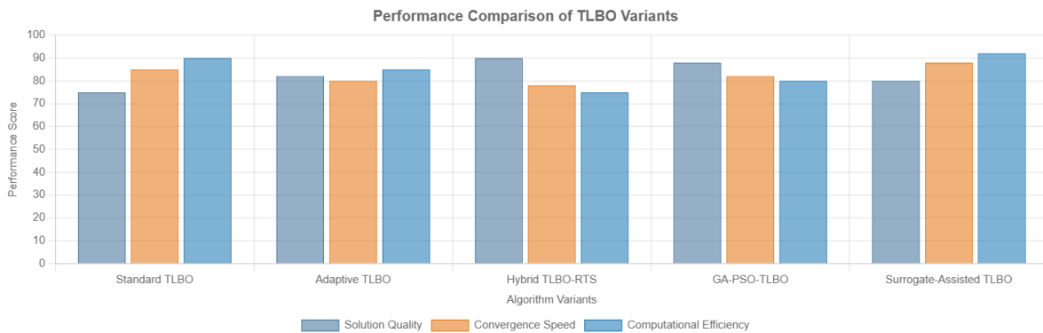
FIGURE 4. TLBO Performance comparison
